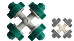
AY-1004B COLOR: GREEN OR GREY PRESSURE: 1.5-3 BAR RADIUS: 0.7-1 M FLOW RATE: 30-35L/H
