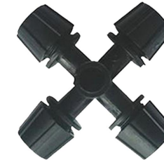
AY-1004F FOUR HEAD FOGGER- BLACK PRESSURE: 1.5-3.5 BAR RADIUS: 0.9-1.1 M FLOW RATE: 30-42 L/H
