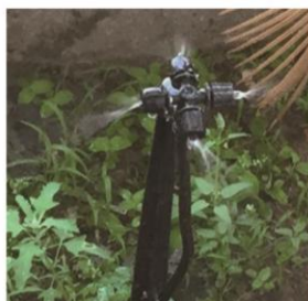
AY-1004B COLOR: GREEN OR GREY PRESSURE: 1.5-3 BAR RADIUS: 0.7-1 M FLOW RATE: 30-35L/H
