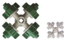
AY-1004 COLOR: GREEN OR WHITE PRESSURE: 1.5-3 BAR RADIUS: 0.7-1 M FLOW RATE: 30-35L/H
