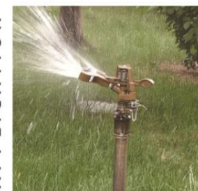
AY-5201 SIZE: 1/2" PRESSURE: 2-3 BAR RADIUS: 3-7 M
